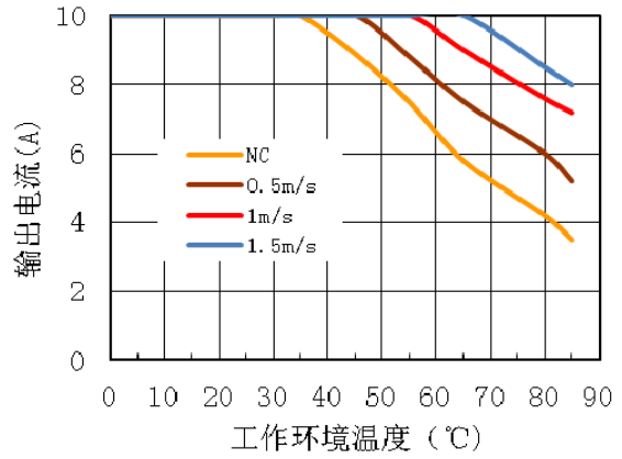
Derating (Vin=12Vdc)
