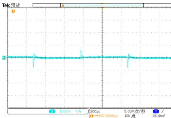
50%~100%~50% load, 0.1A/μs Vin=12Vdc
