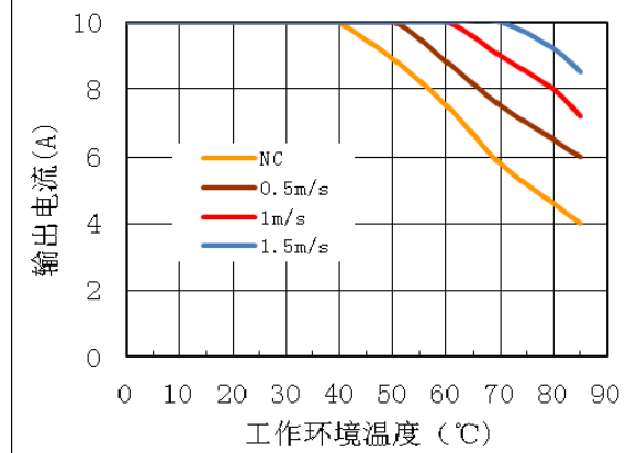
Derating (Vin=12Vdc)
