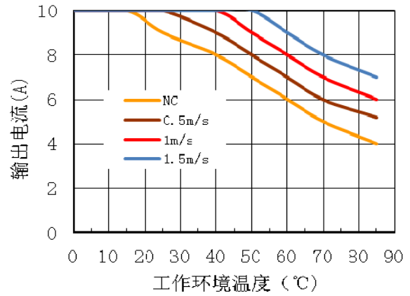
Derating (Vin=12Vdc)
