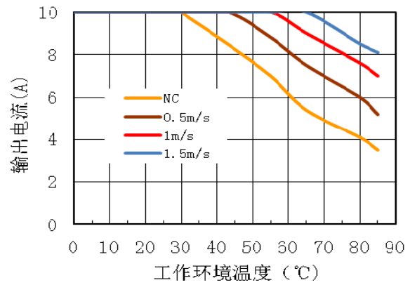
Derating (Vin=12Vdc)
