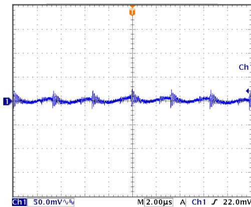
Output Ripple
