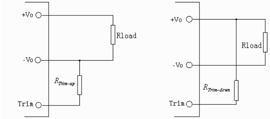
Connection of Trimming Up
