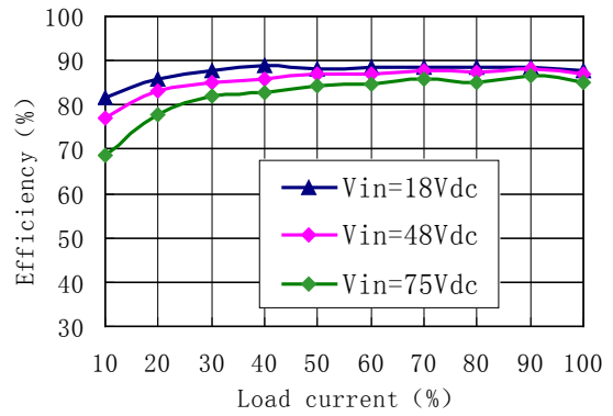
Efficiency vs. Io & Vin
