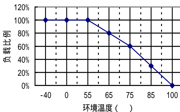
Derating
