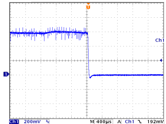
Derating (Vin=12.0Vdc)
