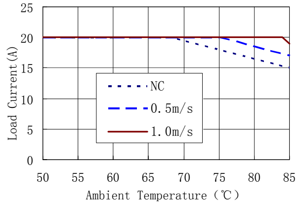
Derating (Vin=12.0Vdc)
