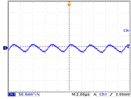
Output Ripple
