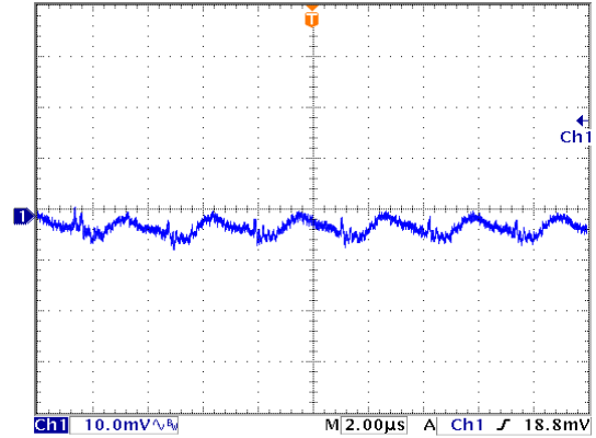
Output Ripple
