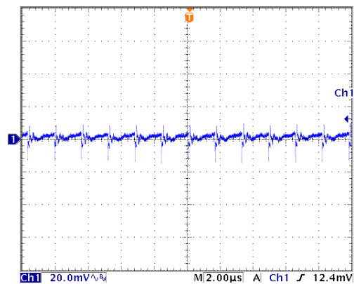
Output Ripple
