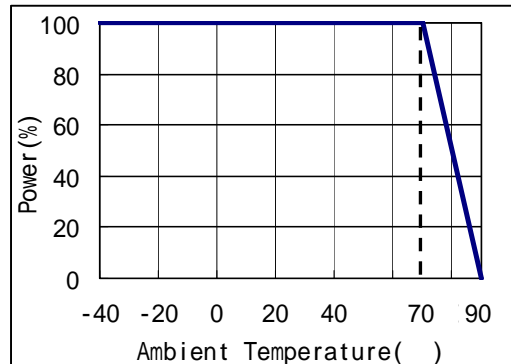
Derating
