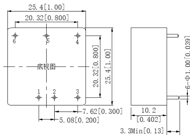
(TH package)
