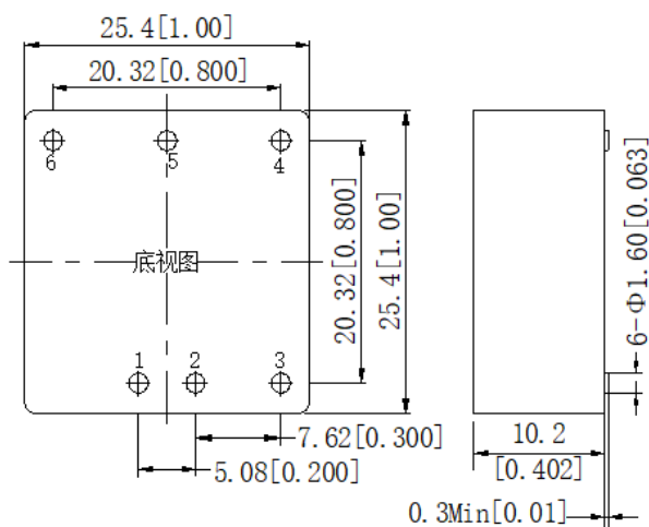
(SMT package)
