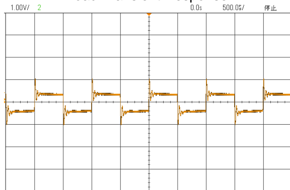
24V in, Load change 0A-5A-0A, 1A/ μ s
