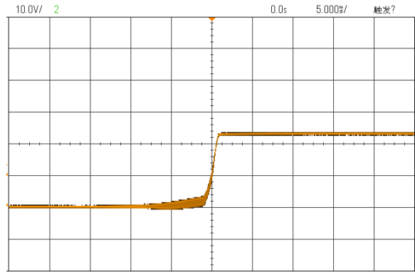
24V in, 8A output with 10 μ F input capacitance and 0 μ F output capacitance
