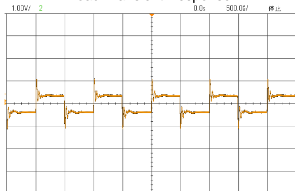
24V in, Load change 5A-10A-5A, 1A/ μ s
