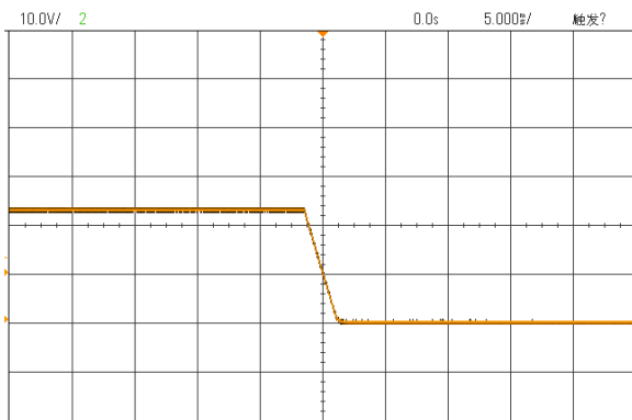
24V in, 8A output with 10 μ F input capacitance and 1000 μ F output capacitance
